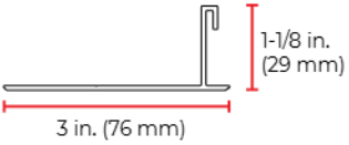
3-in. closure
