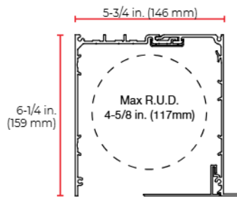
4157 Standard Pocket
