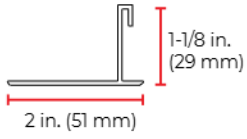
2-in. closure
