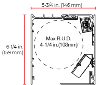
4156 ElectroPocket
