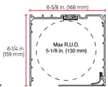
4168 Standard Pocket
