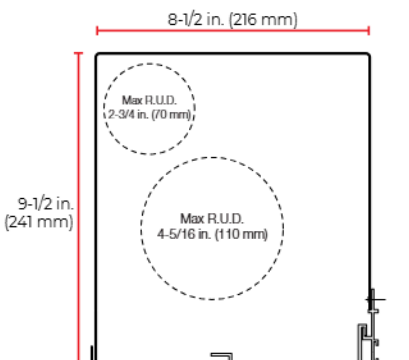
5113 Pocket
