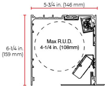
4155 ElectroPocket®
