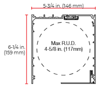
4158 Standard Pocket
